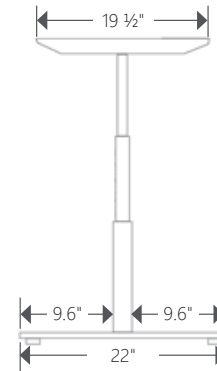
2-Leg Small Frame [CGSA-2LS] Side View
