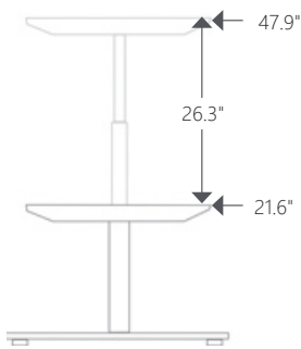
2-Leg Small and 2-Leg Frame [CGSA-2LS & CGSA-2L] Height Range
