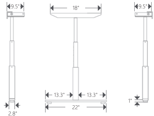
3-Leg Modular Frame [CGSAMOD-3L-120] Front View*
