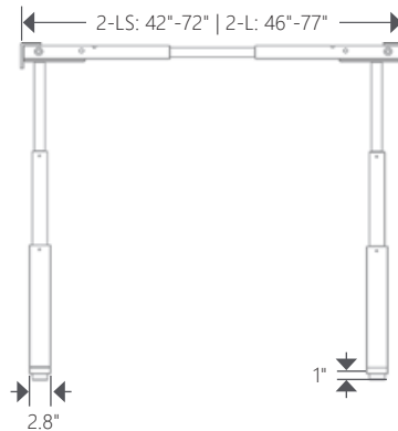
2-Leg Small and 2-Leg Frame [CGSA-2LS & CGSA-2L] Front View
