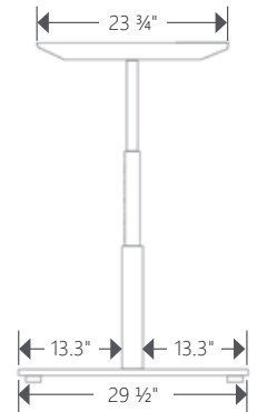
2-Leg Frame [CGSA-2L] Side View
