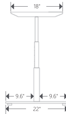
2-Leg Small Modular [CGSAMOD-2LS] Side View
