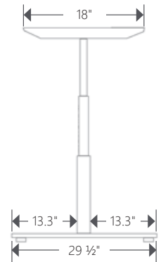
2-Leg Modular [CGSAMOD-2L] Side View
