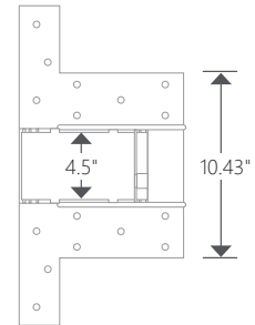
2-Leg Modular Frames [CGSAMOD-2LS & CGSA MOD-2L] Top Down View
