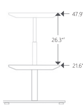
3-Leg Modular Frame [CGSAMOD-3L-120] Height Range
